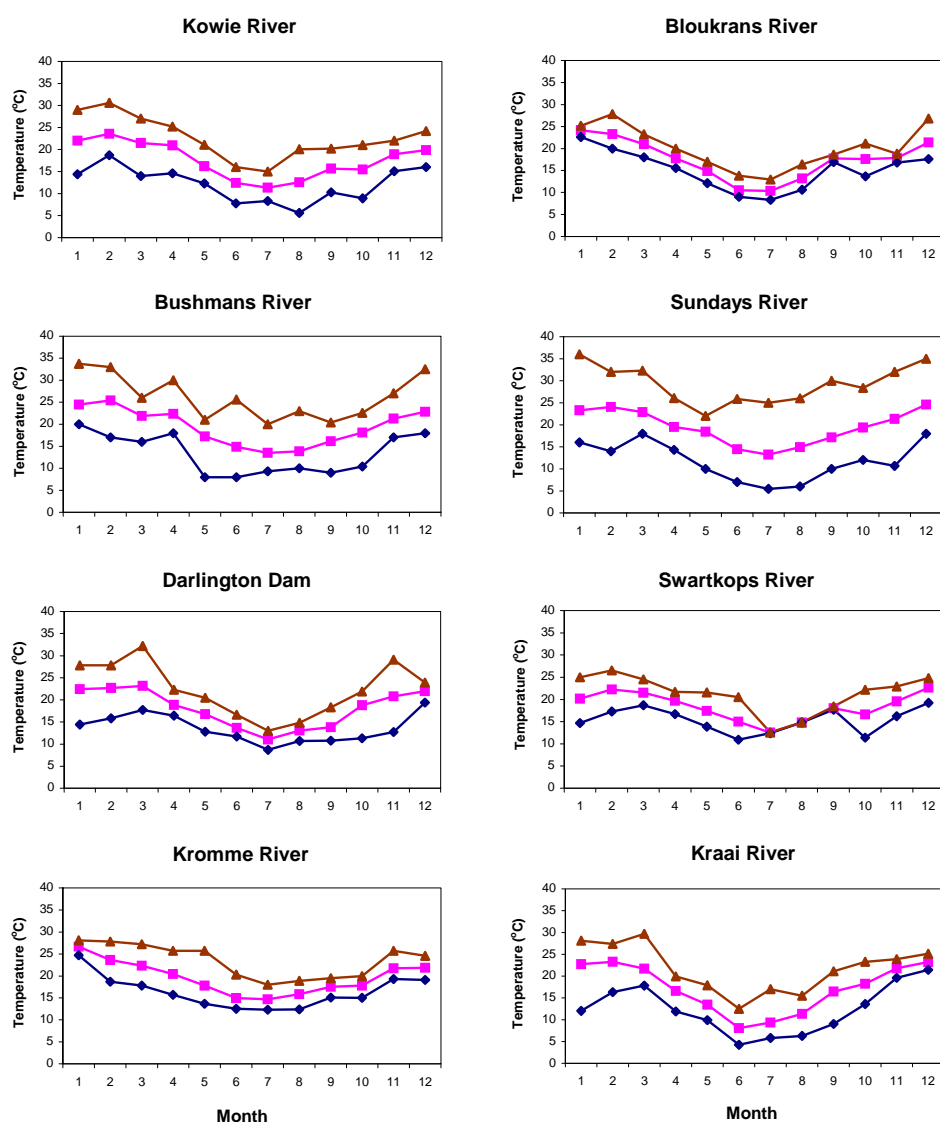
Figure 3. Temperature profiles for 20 selected water bodies in the Eastern Cape, derived from the DWA - Hydrological Services Department Database for 1974 to 2007. The graphs show the monthly temperatures, as means of all data (■), maximum recorded (▲), and minimum recorded (◆).
